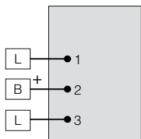
SPDT On-Off-On
